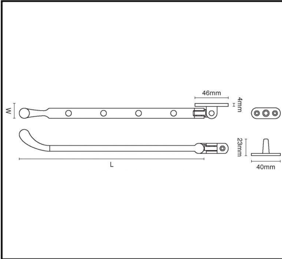
Bulb End Casement Stay 1791
